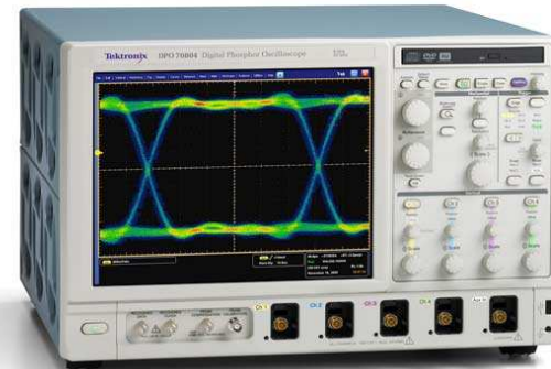
DPO70804 for HDMI PHY Tests
